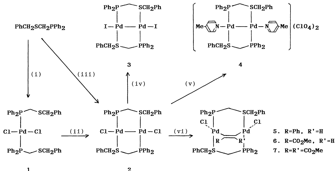
Scheme 1. (i) \text{Na}_2[\text{PdCl}_4] . (ii) [\text{Pd}(\text{dba})_2] . (iii) [\text{PdCl}_2(\text{NCMe})_2] and [\text{Pd}(\text{dba})_2] . (iv) \text{NaI} . (v) 4-MePy and \text{AgClO}_4 . (vi) \text{RC}\equiv\text{CR}' .
